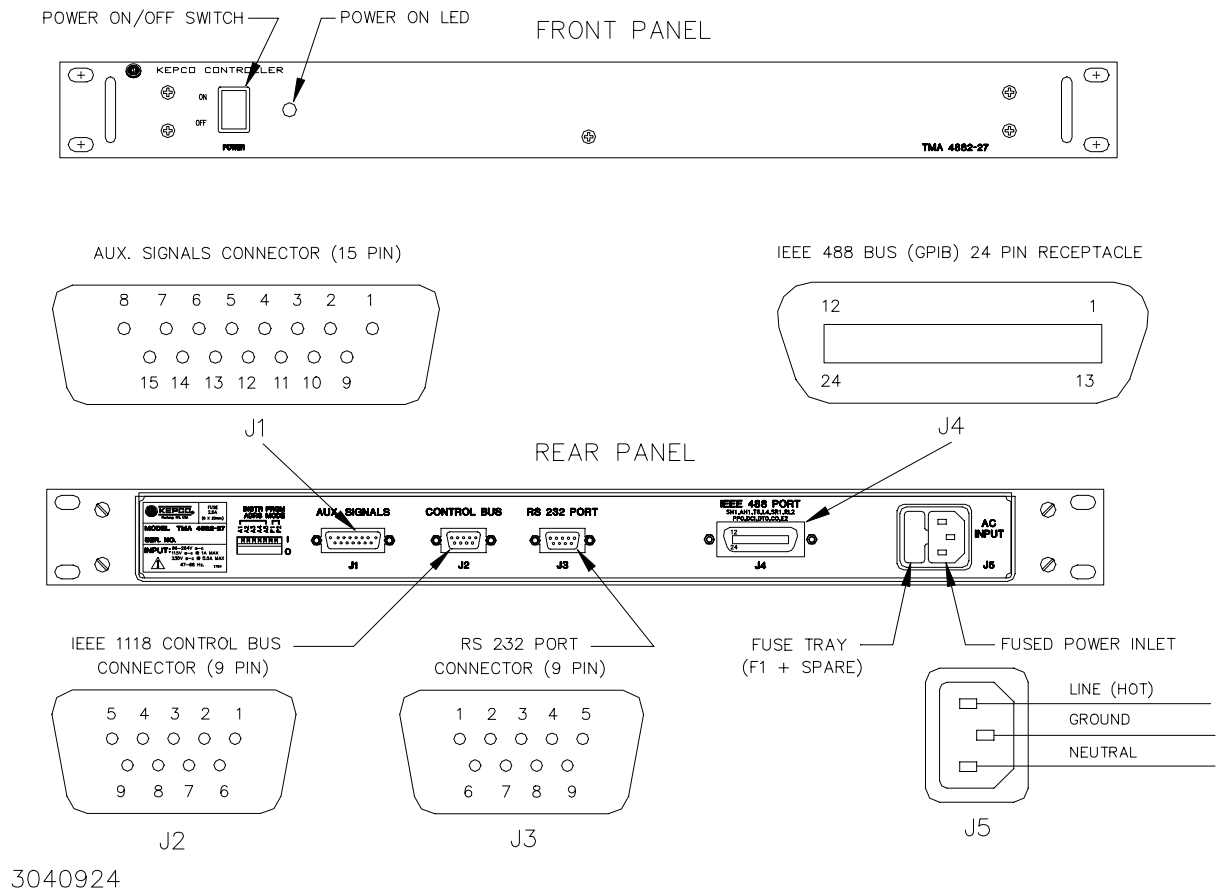
FIGURE 2-2. TMA 4882-27 FRONT AND REAR PANELS
