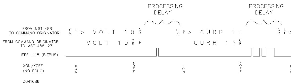
FIGURE 3-1. RS 232 IMPLEMENTATION
