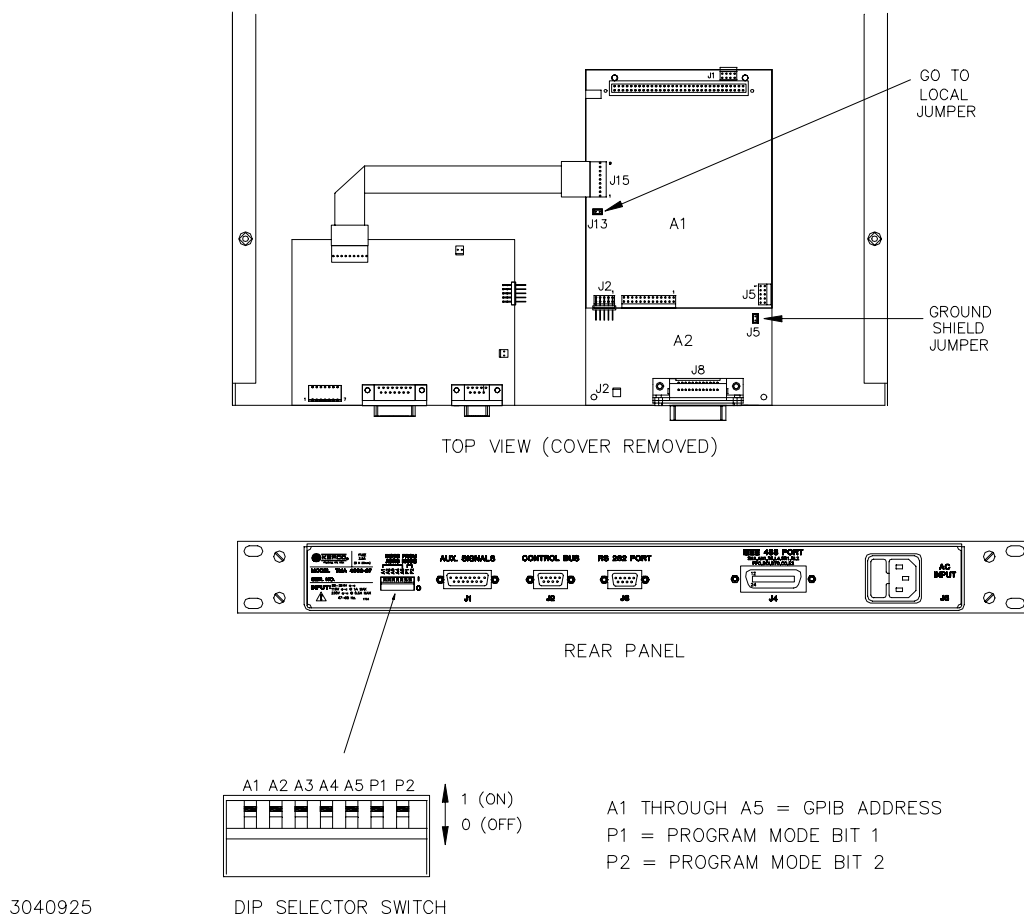
FIGURE 2-1. TMA 4882-27 CONFIGURATION CONTROLS
