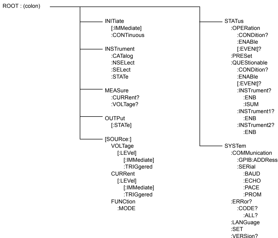
FIGURE 3-2. TREE DIAGRAM OF SCPI COMMANDS USED WITH TMA 4882-27 CONTROLLER
